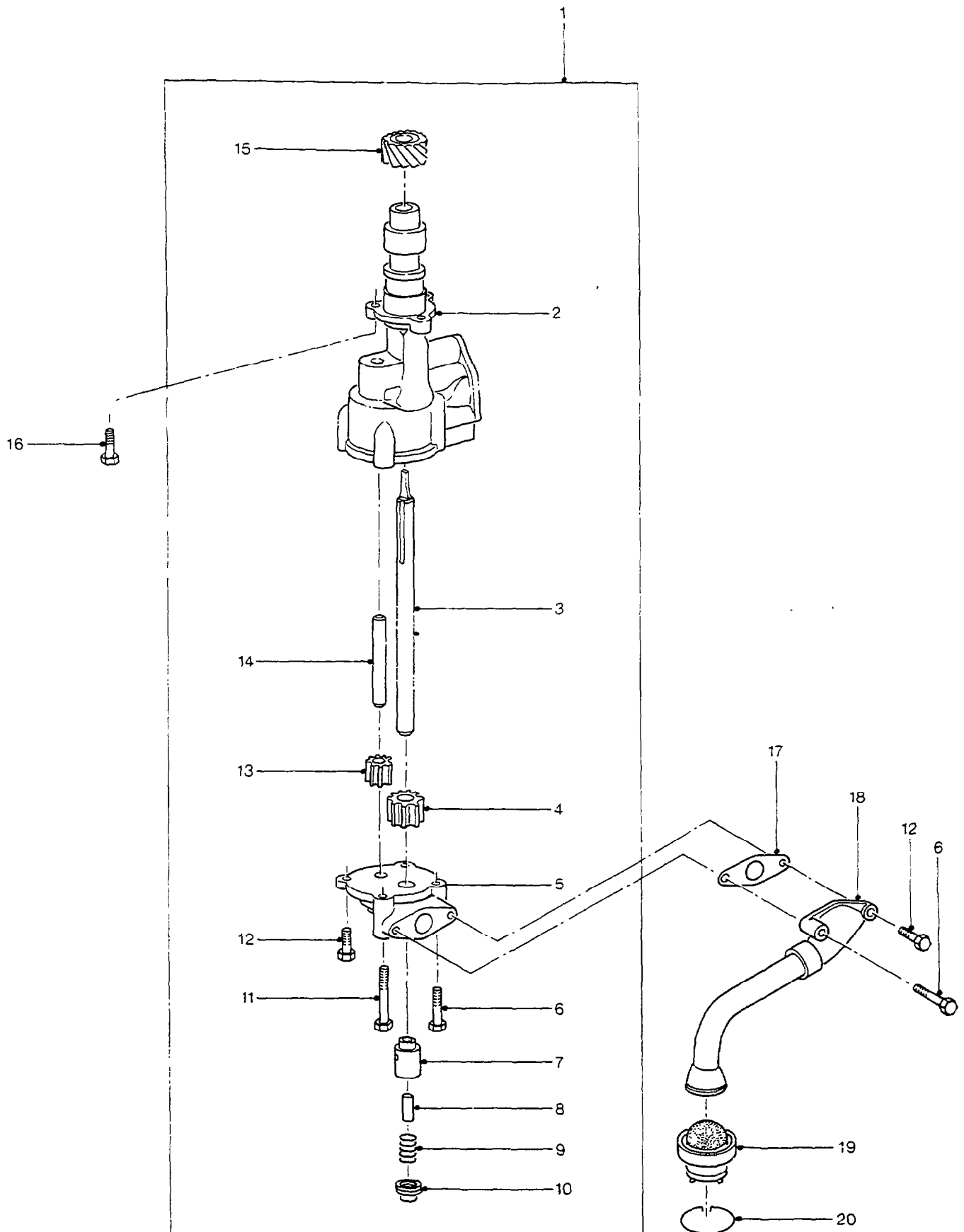
OIL PUMP ASSEMBLY
