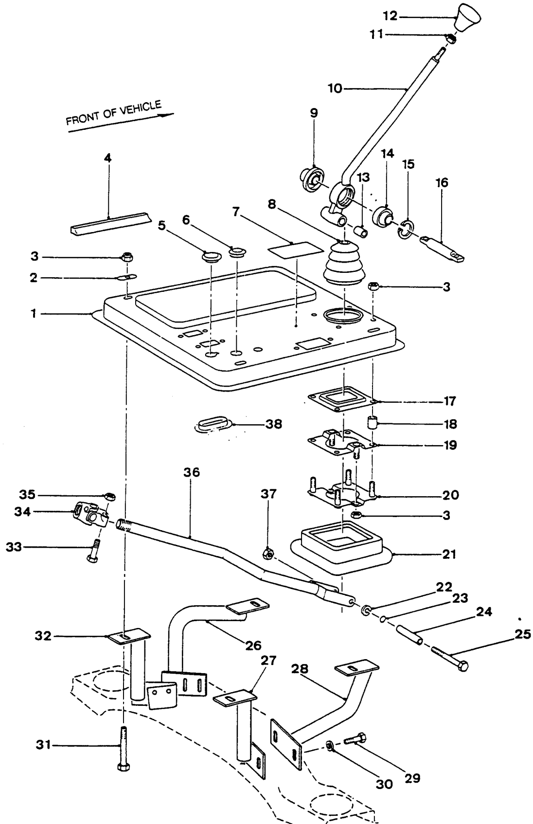
GEAR SHIFT LEVER AND LINKAGE
