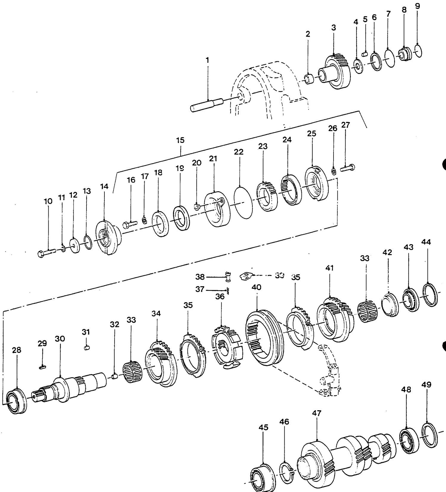
INPUT GEARTRAIN AND COUNTERSHAFT
