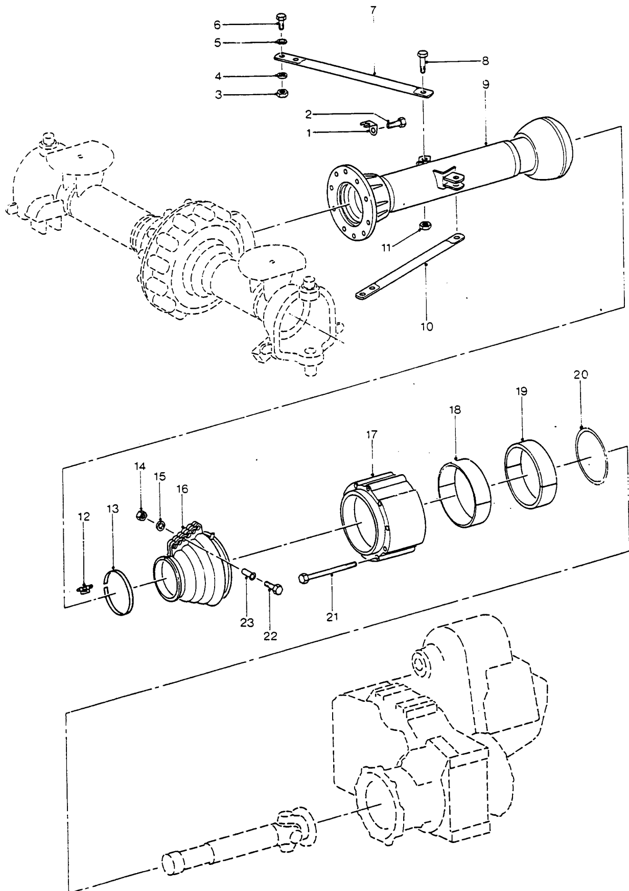
TORQUE TUBE HOUSINGS
