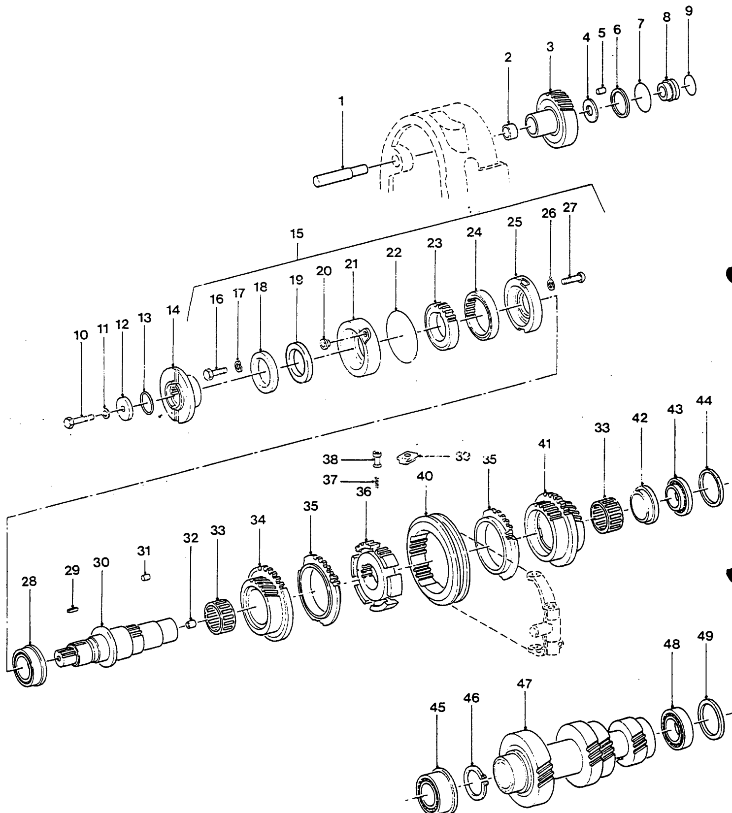
INPUT GEARTRAIN AND COUNTERSHAFT
