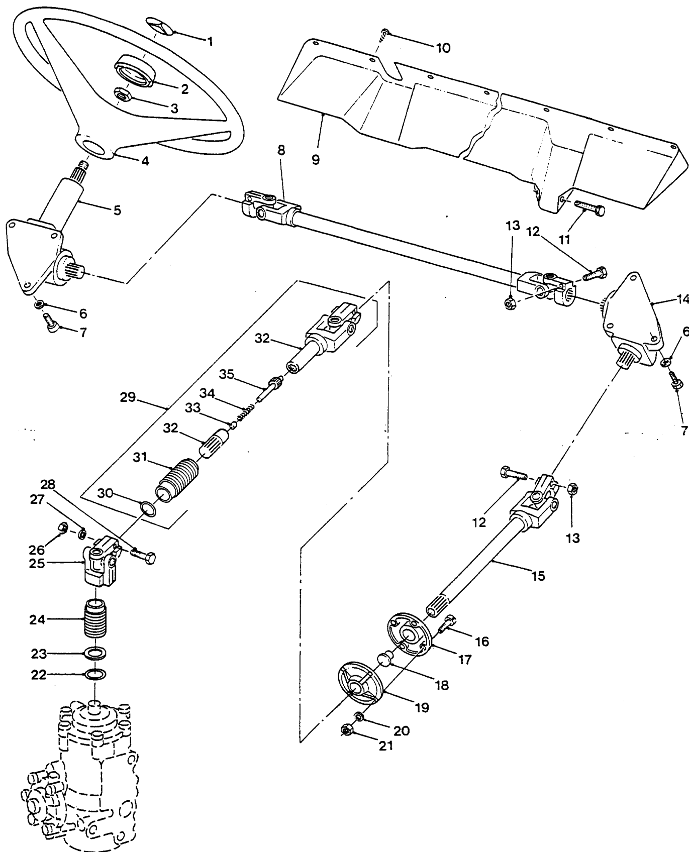
STEERING WHEEL, COLUMN DRIVE SHAFTS AND DRAG LINK
