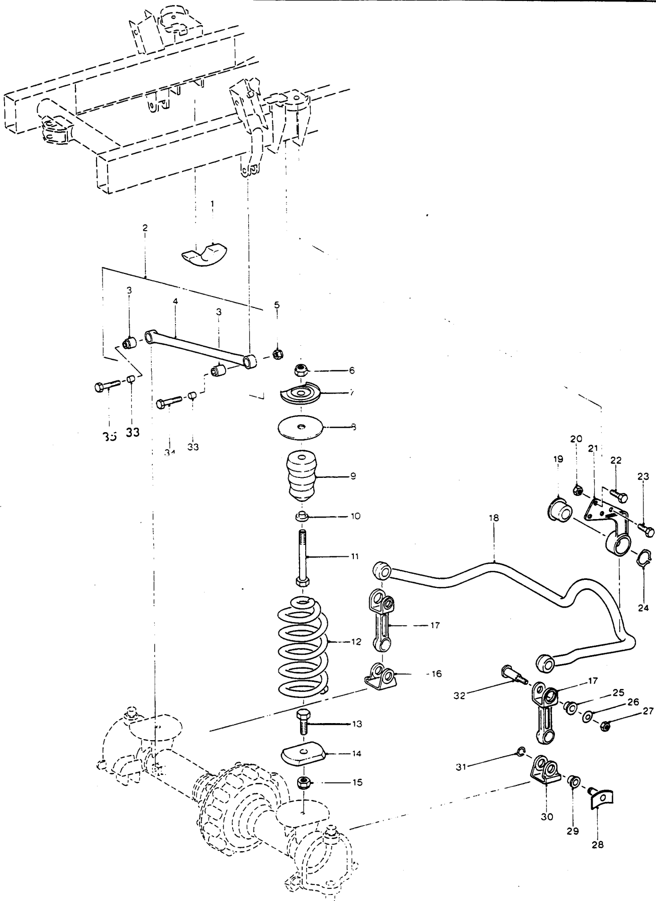
FRONT SPRINGS/STABILISER RODS
