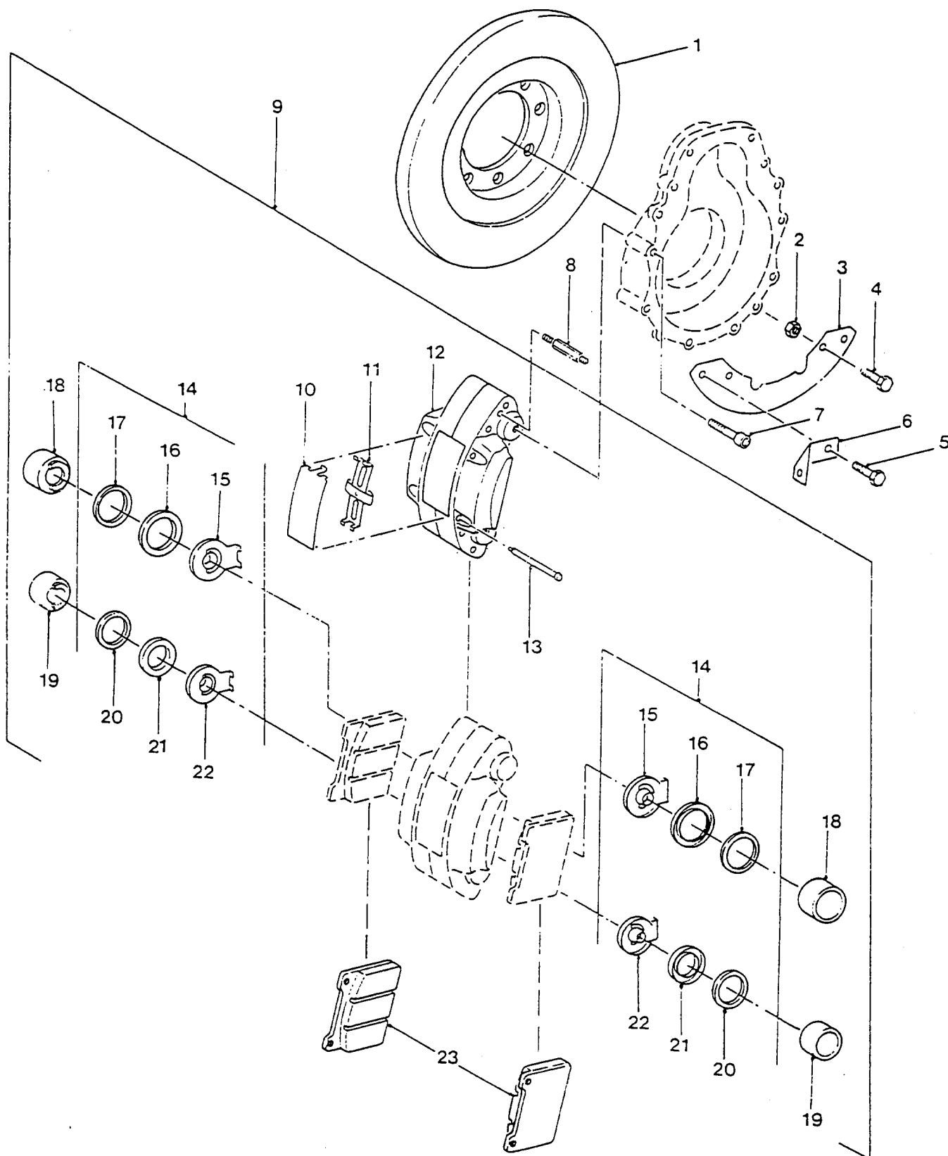
BRAKE DISCS, CALIPERS AND PADS, FRONT AXLE
