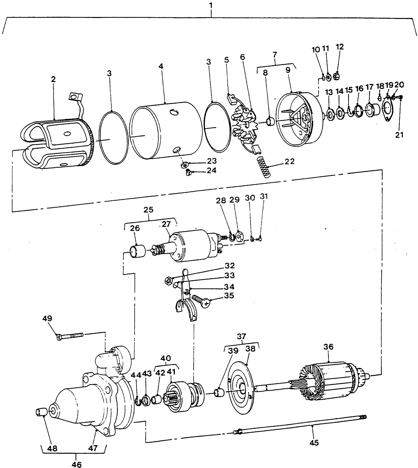
STARTER MOTOR AND SOLENOID ASSEMBLY (LATE MODEL)
