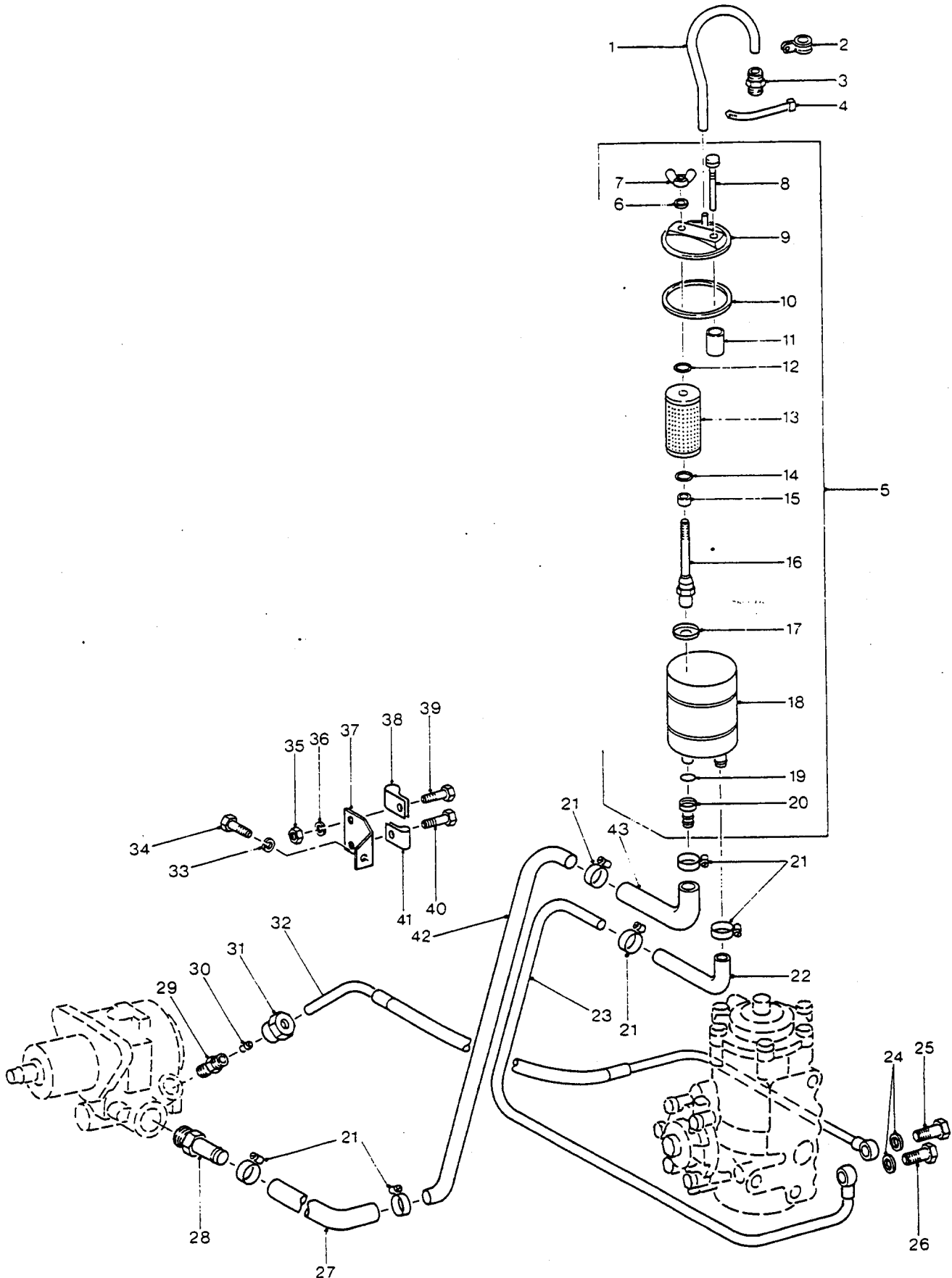
POWER STEERING RESERVOIR AND PIPING
