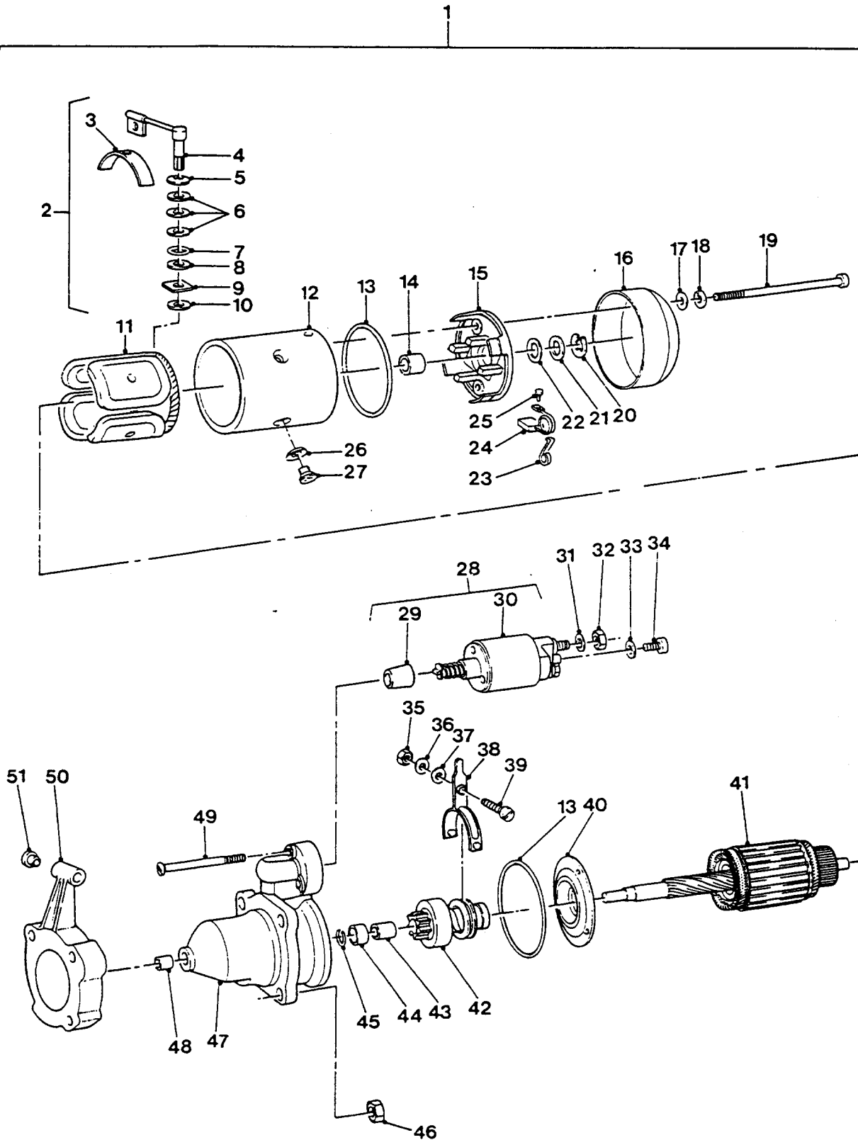
STARTER MOTOR AND SOLENOID ASSEMBLY (EARLY MODEL)
