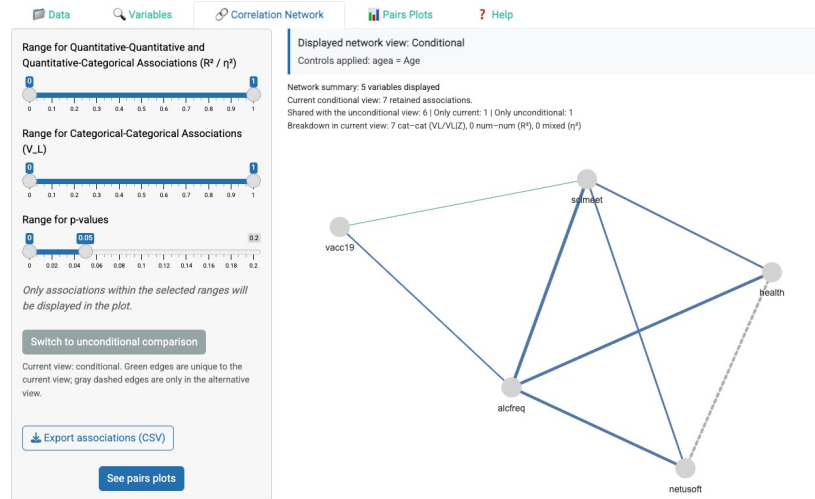
Conditional association network with age of respondent ( agea ) as control.
