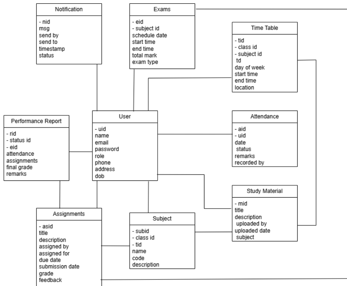
Figure 4.4: Schema diagram for EduNest School management system
