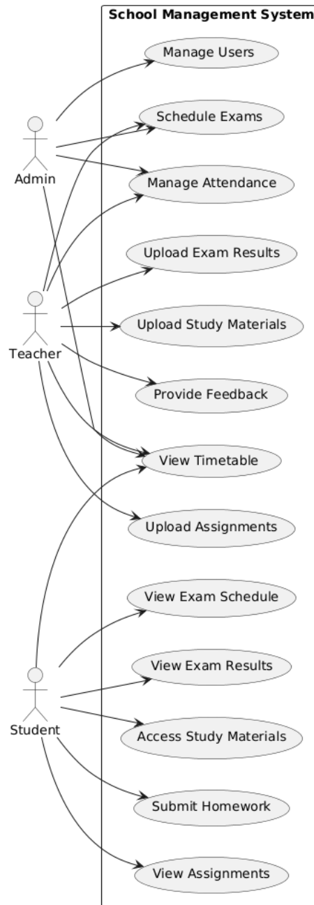
Figure 4.1: Use case diagram of EduNest school management system
