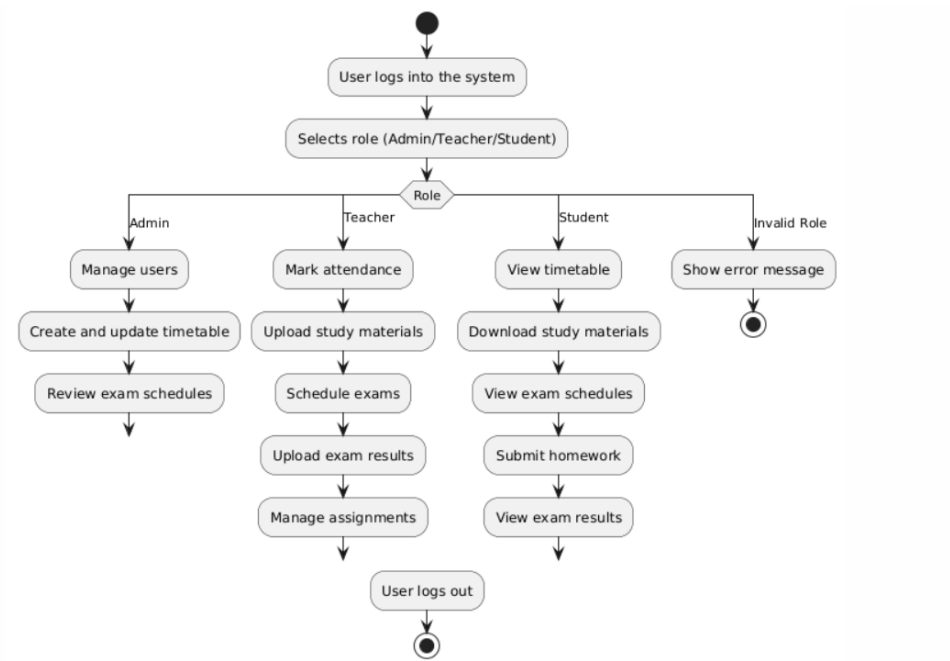
Figure 4.2: Activity diagram of EduNest school management system
