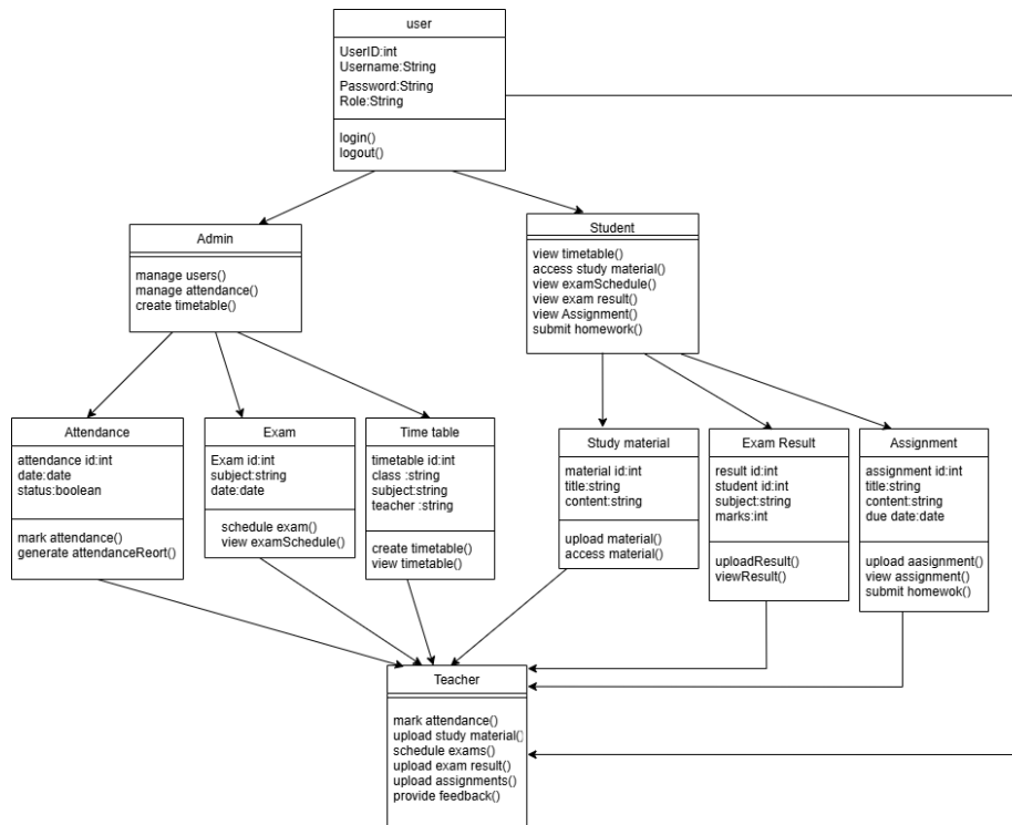
Figure 4.3: class diagram of the EduNest school management system
