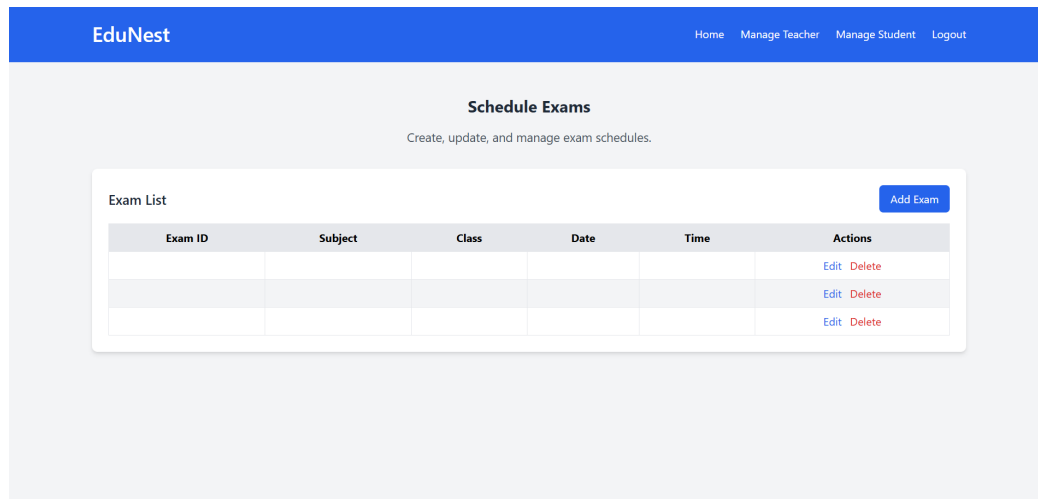
Figure 4.9: Schedule exam
