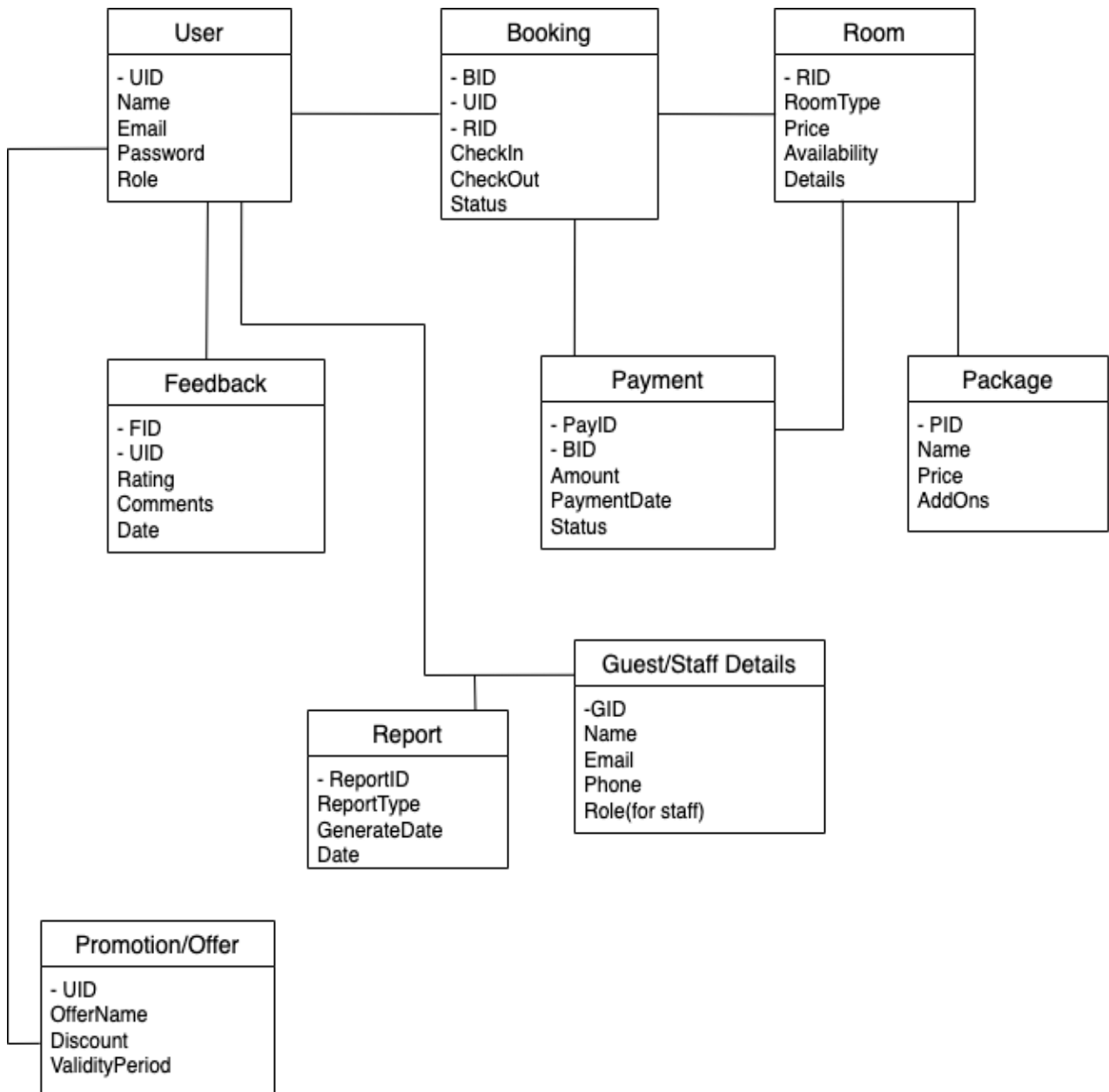
Figure 4.4: Schema Diagram
