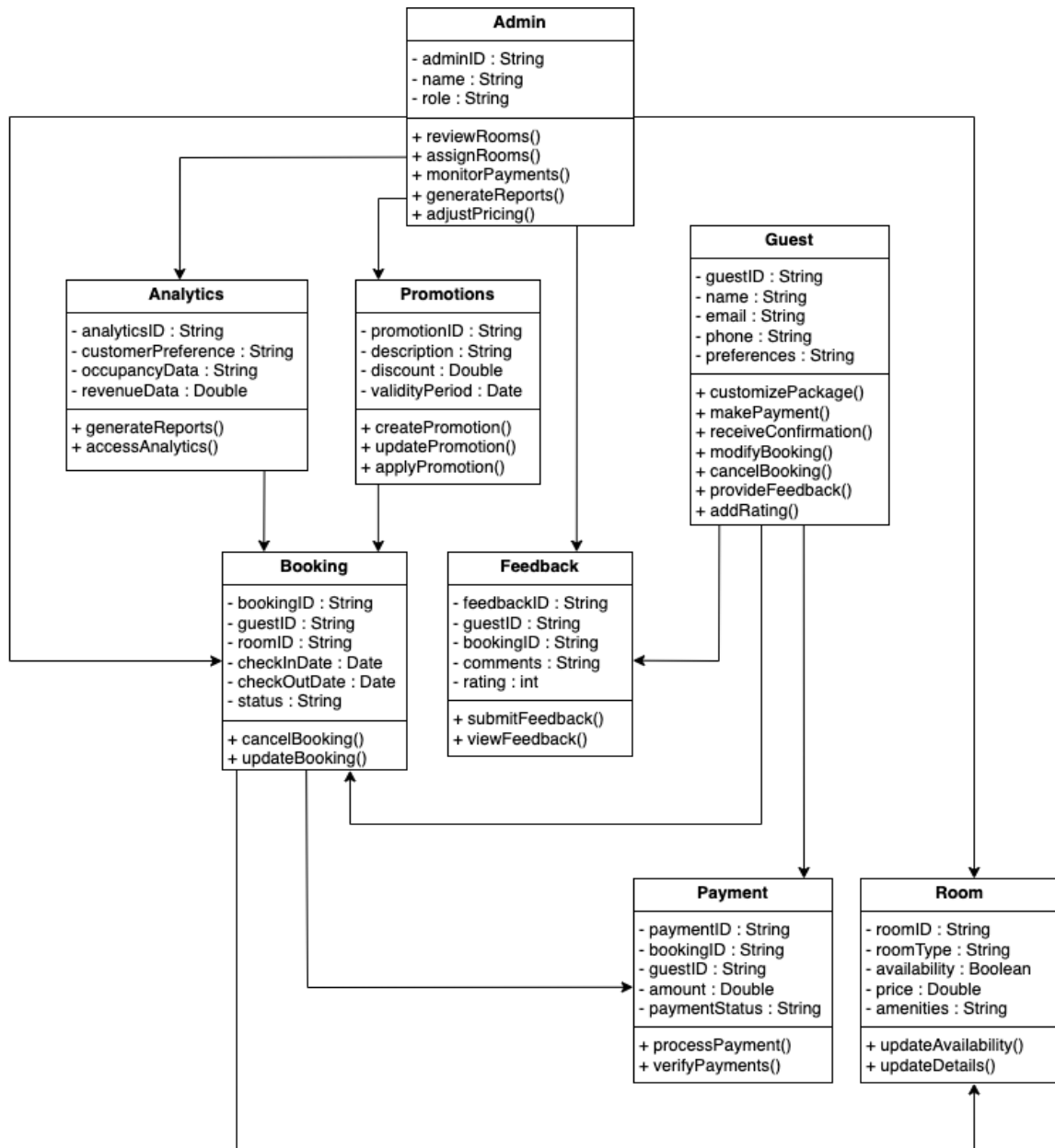
Figure 4.3: Class Diagram
