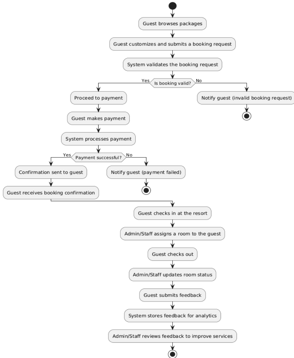
Figure 4.2: Activity Diagram
