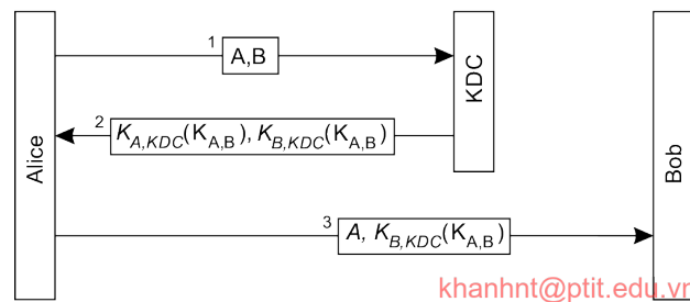
Figure 9.10: Using a ticket and letting Alice set up a connection to Bob.
