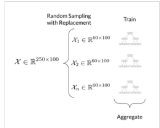
Illustration of training a Random Forest model. The training dataset (in this case, of 250 rows and 100 columns) is randomly sampled with replacement n times. Then, a decision tree is trained on each sample. Finally, for prediction, the results of all n trees are aggregated to produce a final decision.
