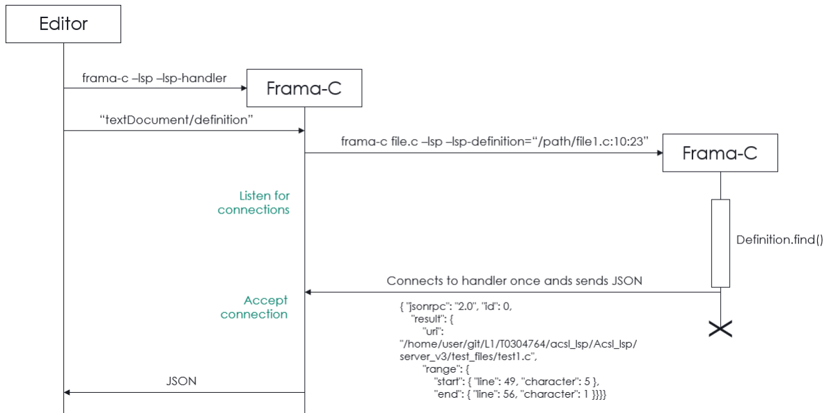
Figure 9: LSP plug-in example of handler mode usage sequence diagram
