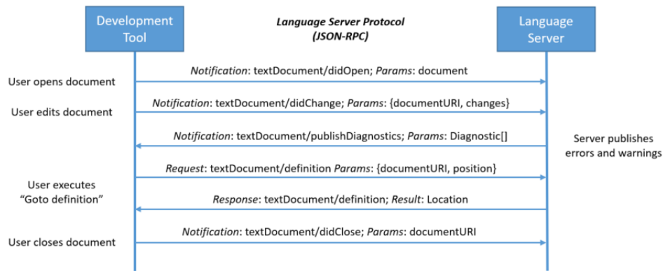
Figure 3: Language Server Protocol sequence diagram: example of an interaction flow between client and server
