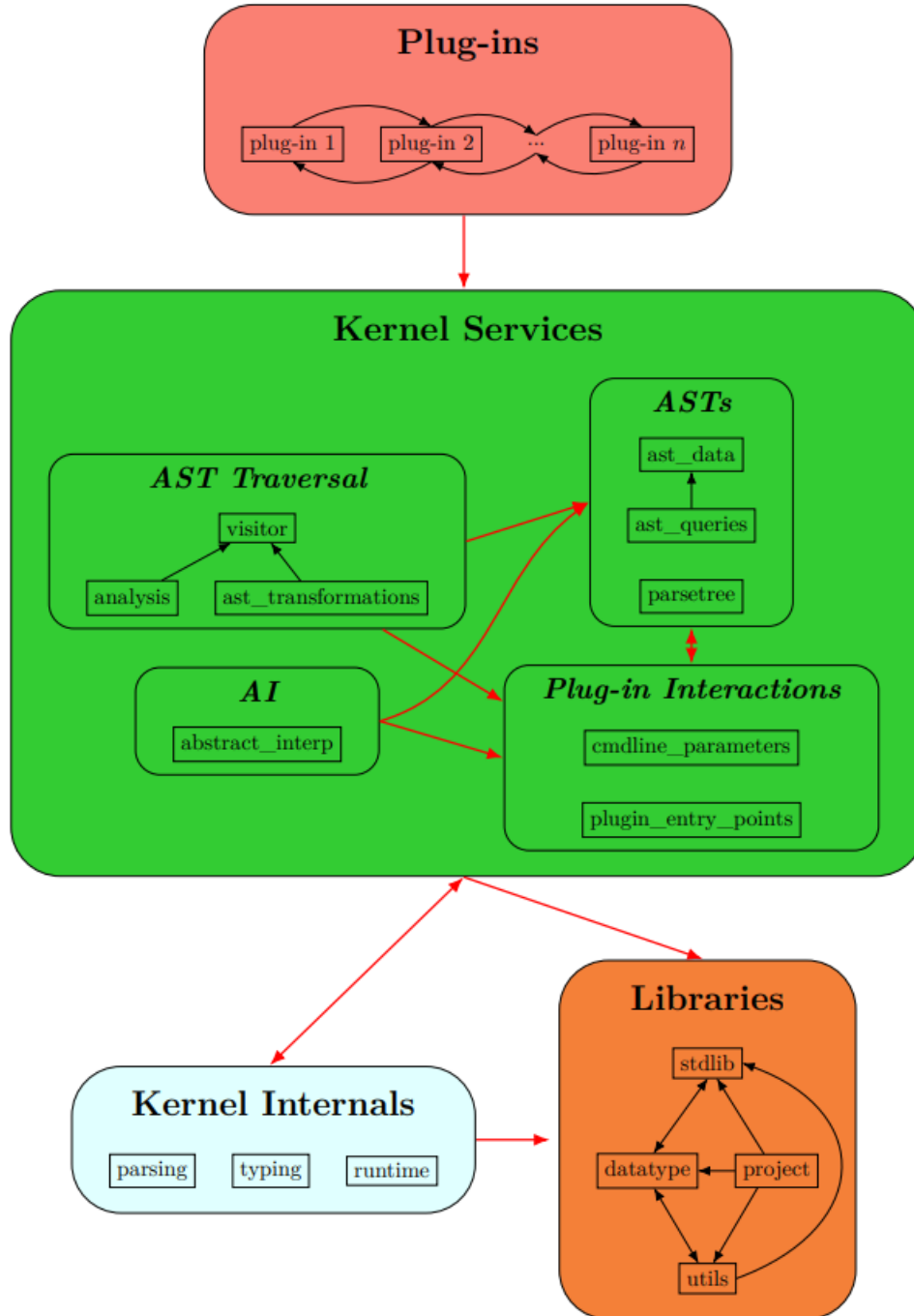
Figure 4: Frama-C Architecture Design
