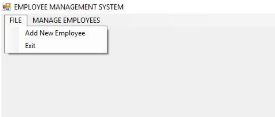
FIGURE 2: File menu
