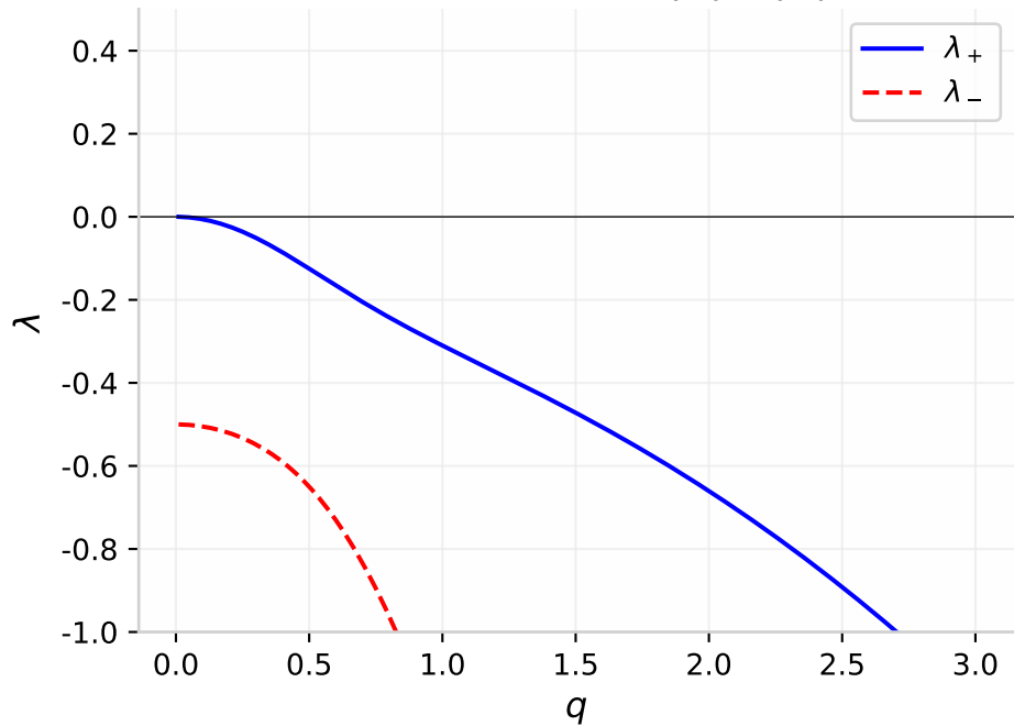
Stable: \alpha = -0.2, D|\mu| > |\alpha|\rho_0
