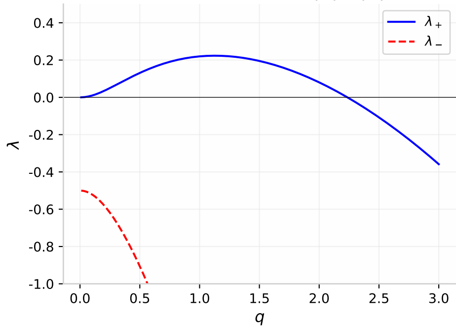
Unstable: \alpha = -1.0, D|\mu| < |\alpha|\rho_0
