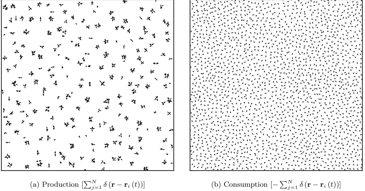
Figure 1: Snapshots of particle configurations for (a) production and (b) consumption of chemoattractant. The parameters are \alpha = 0.5 , D = 0.001 , D_c = 0.1 , \mu = -0.001 , and N = 2000 particles in an L = 20 domain. The positions and velocity direction of the particles are shown as arrows.
