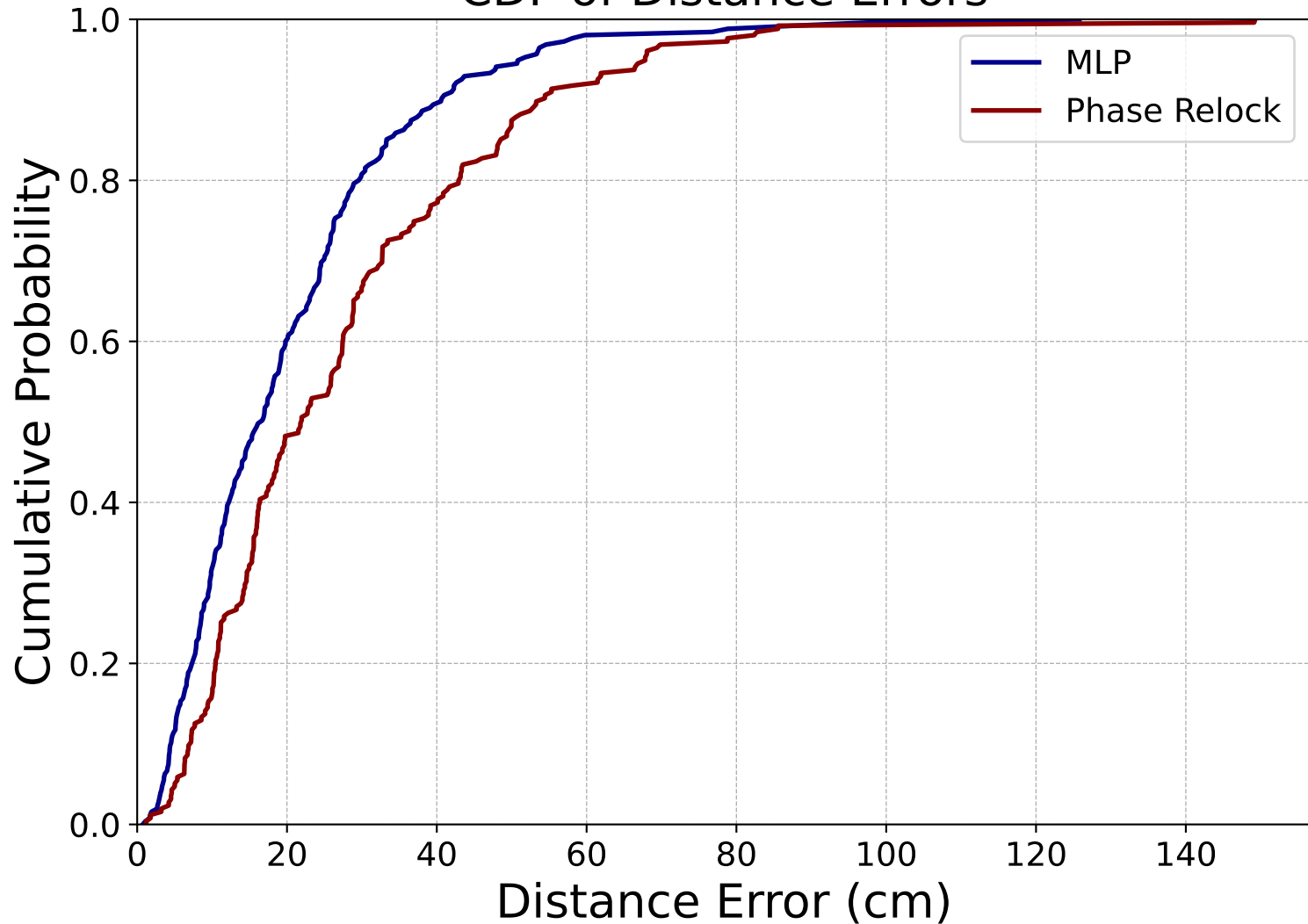
CDF of Distance Errors
