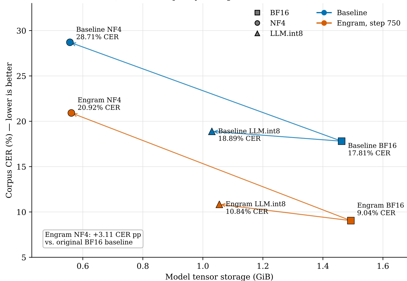
Quantization quality-storage trade-offs (N = 300)
