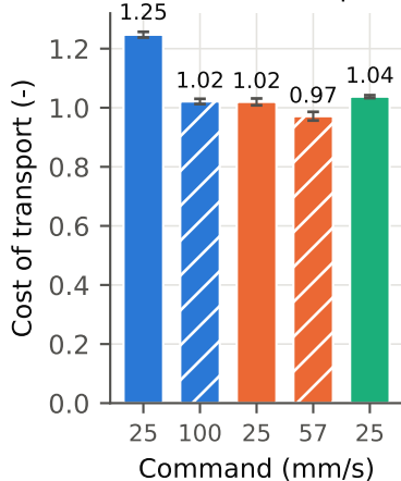
(c) Cost of transport
