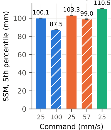
(b) Static stability margin
