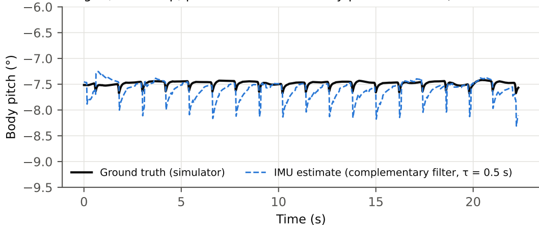
Wave gait, 15° ramp, posture control on: body pitch estimate (RMS error 0.20°)
