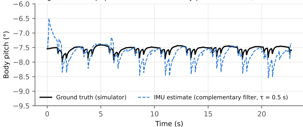
Wave gait, 15° ramp, posture control on: body pitch estimate (RMS error 0.28°)
