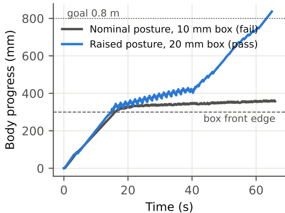
(a) Tripod body progress
