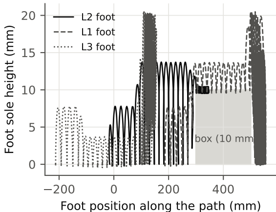
(b) Left feet, nominal posture, 10 mm box
