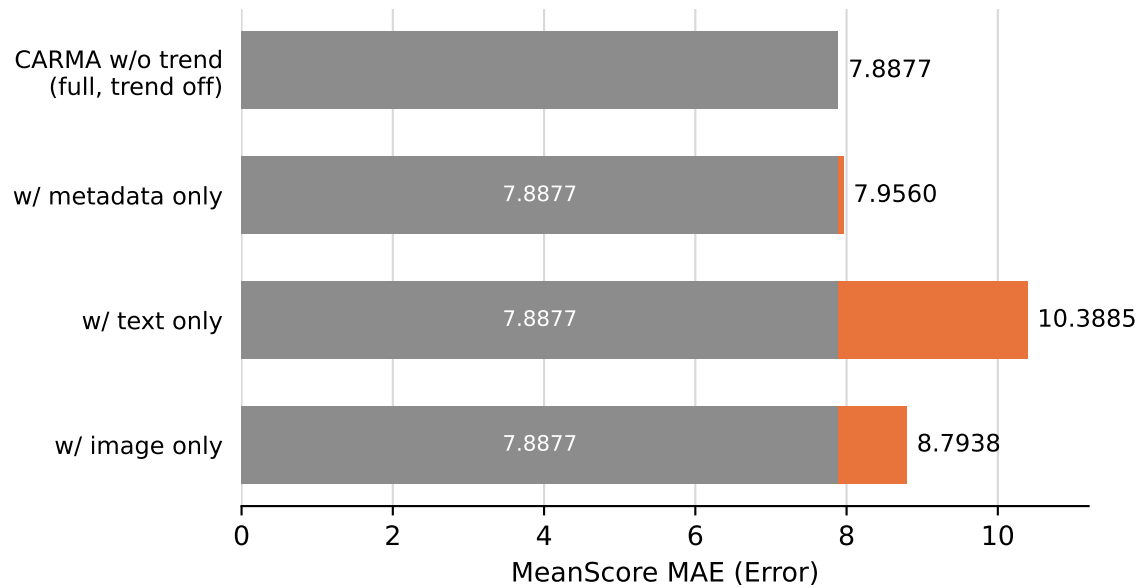
MeanScore
