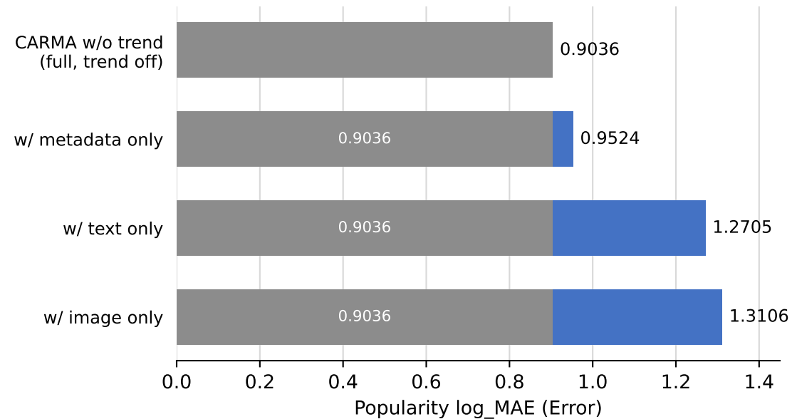
Popularity
