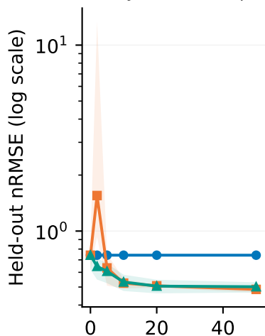
Phenylethanol — pls
