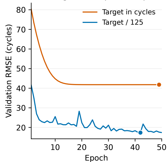
a Original 50-epoch recipe
