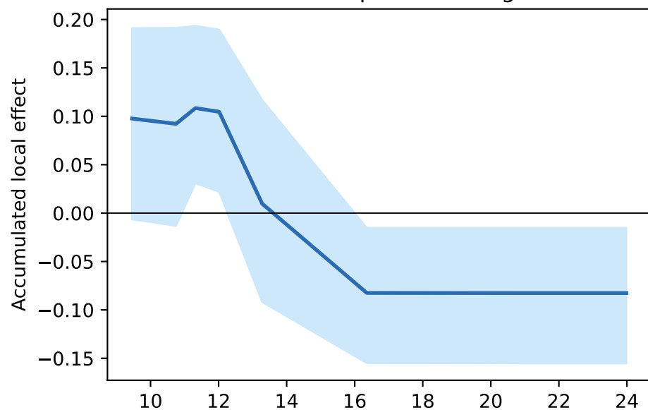
Mean temperature, warmest quarter
