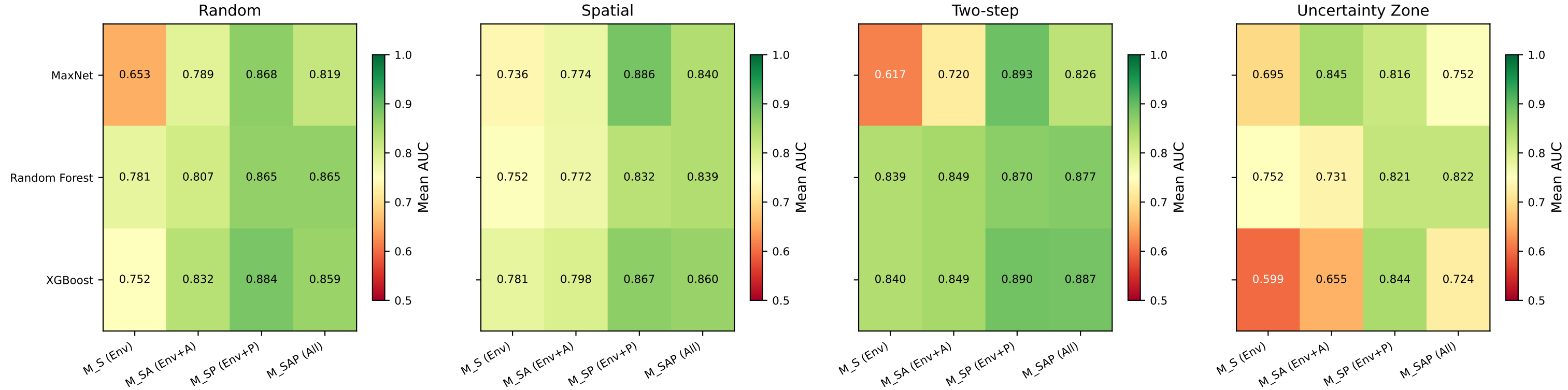
Mean AUC-ROC: Algorithm × Feature Set × PA Method
