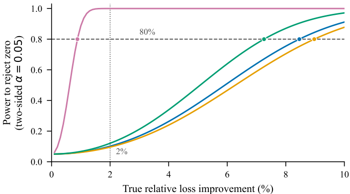
(c) Fresh purged pilot: equivalence test
