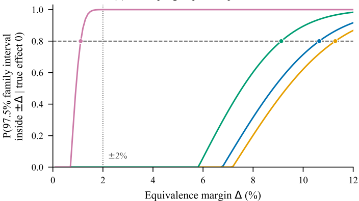
(c) Fresh purged pilot: equivalence test
