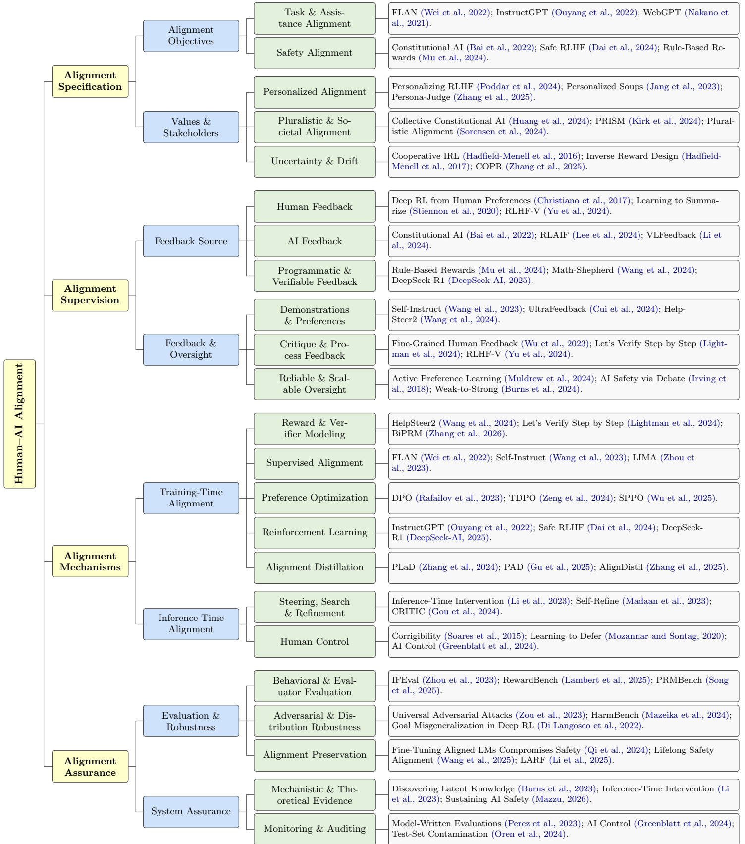
Figure 1: A compact taxonomy of Human-AI Alignment organized along four complementary dimensions and 23 terminal categories. Each gray box lists three illustrative references, while the accompanying mapping retains the full bibliography. Categories are non-exclusive. Demonstrations and preferences include pairwise comparisons, scalar ratings, and multi-attribute judgments. Mechanistic and theoretical evidence is interpreted under the assumptions of the corresponding analyses, while process-verifier quality is assessed within behavioral and evaluator evaluation.
