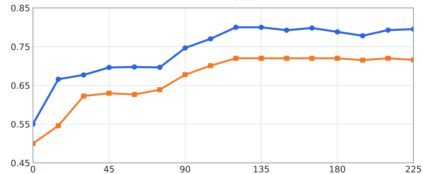
MATH-500
