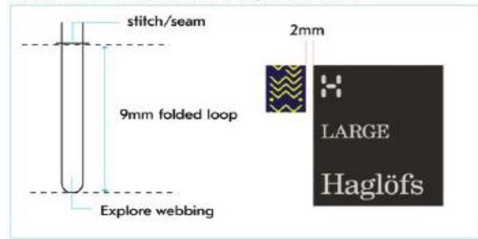
Application of explore webbing to size label
