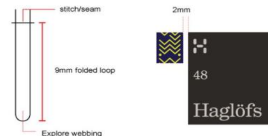
Application of explore webbing to size label
