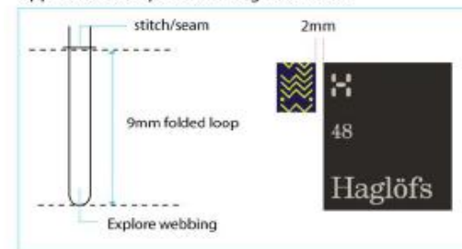
Application of explore webbing to size label
