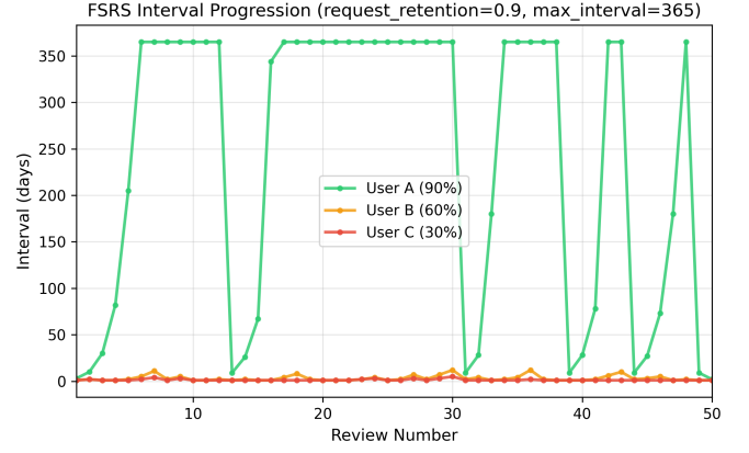
Fig. 6. FSRS interval progression over 50 reviews for three simulated user profiles. User A (90%) reaches the 365-day maximum; Users B and C remain at short intervals, demonstrating adaptive difficulty sensitivity.
