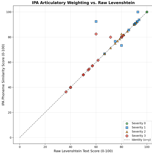
Fig. 5. IPA phoneme similarity versus raw Levenshtein text score. Points deviating from the identity line demonstrate the IPA metric’s discriminatory advantage: same-class phoneme substitutions (e.g., fricative to fricative) are penalized less severely than cross-class substitutions, despite having identical raw edit distances.
