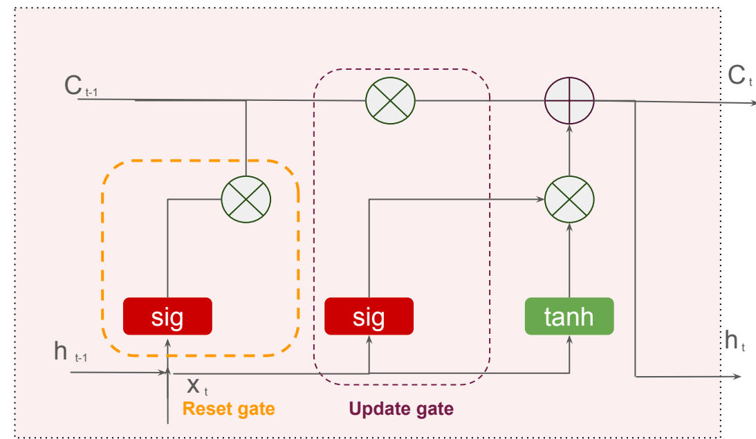
Gated Recurrent Unit (GRU)
