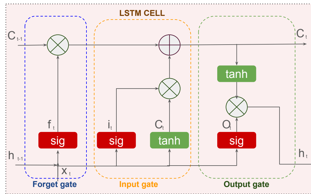
Long Short-Term Memory (LSTM)
