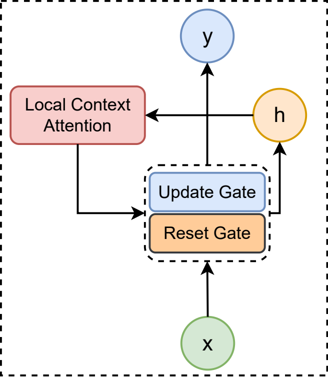
Local Context Attention Gated Recurrent Unit ( LARGU )
