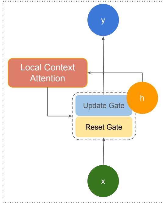
Local Context Attention Gated Recurrent Unit (LAGRU)
