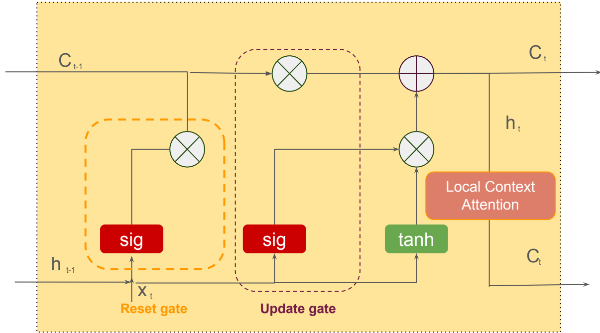
Transform hidden vector to new vector in LAGRU model
