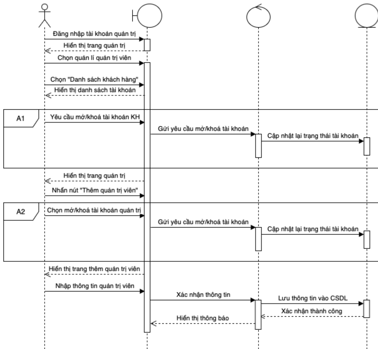
Figure 7: Sequence chart for user management function
