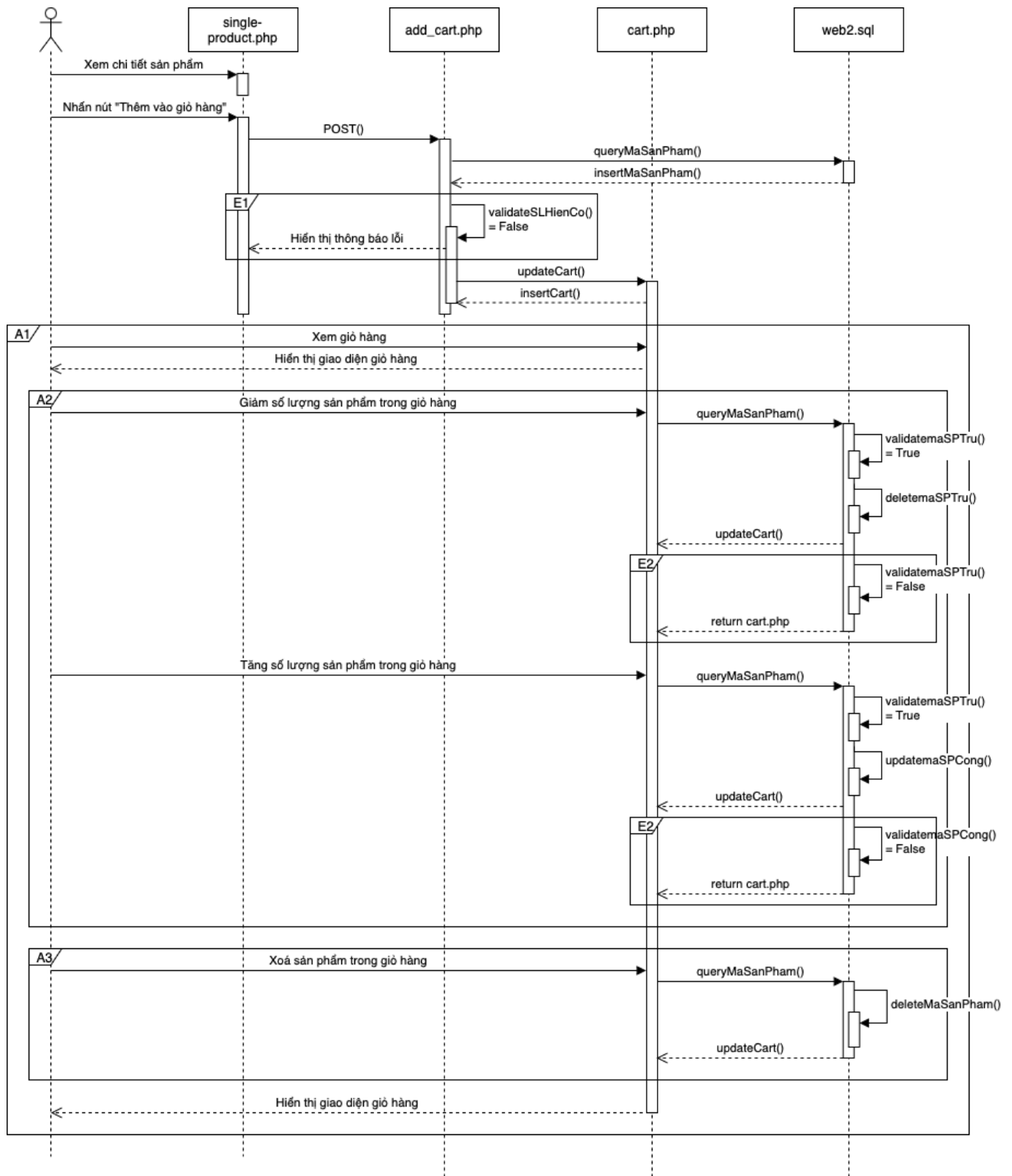
Figure 56: The sequence model of the shopping cart function
