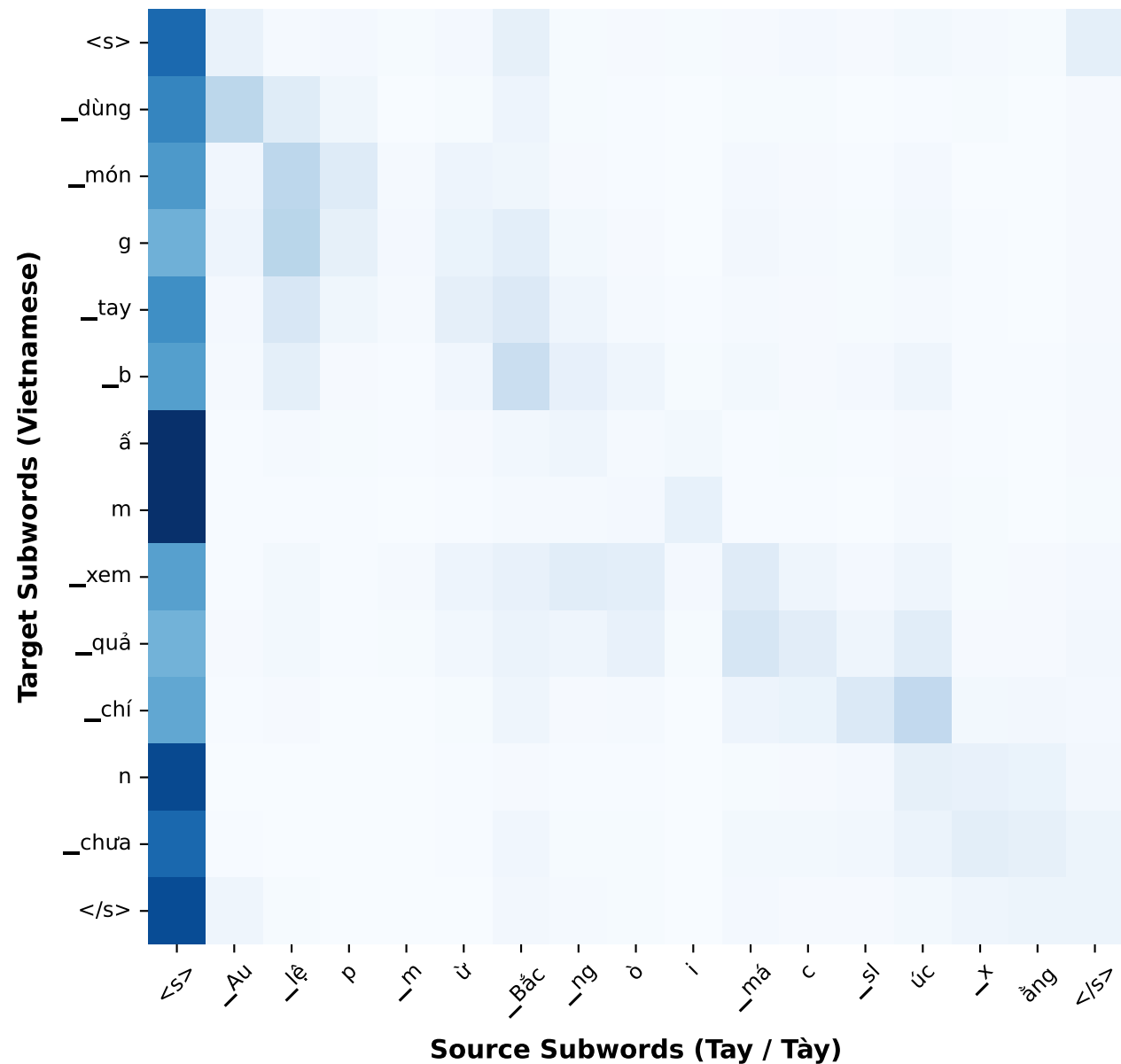
(a) Vanilla BARTpho (Baseline)
