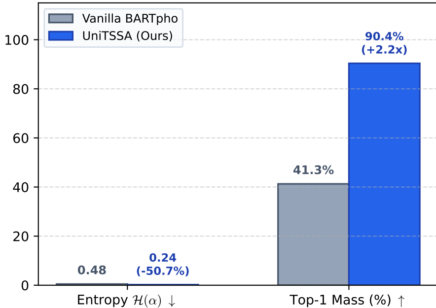
(a) Attention Concentration (Rhade)
