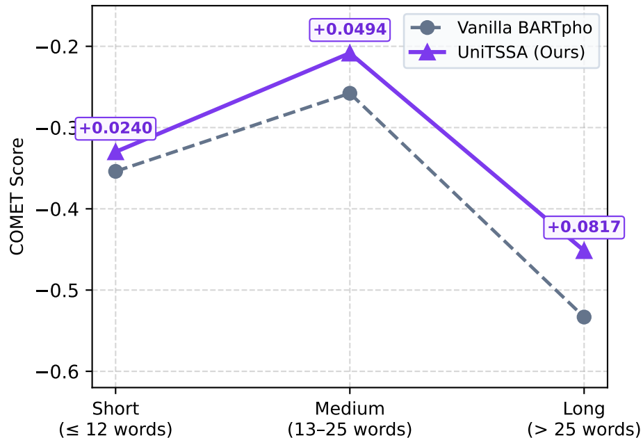
(b) COMET Semantic Fidelity Across Length
