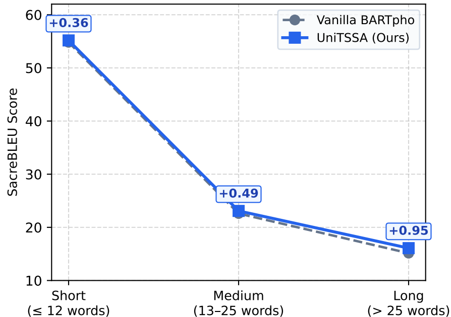
(a) BLEU Score Across Length Buckets
