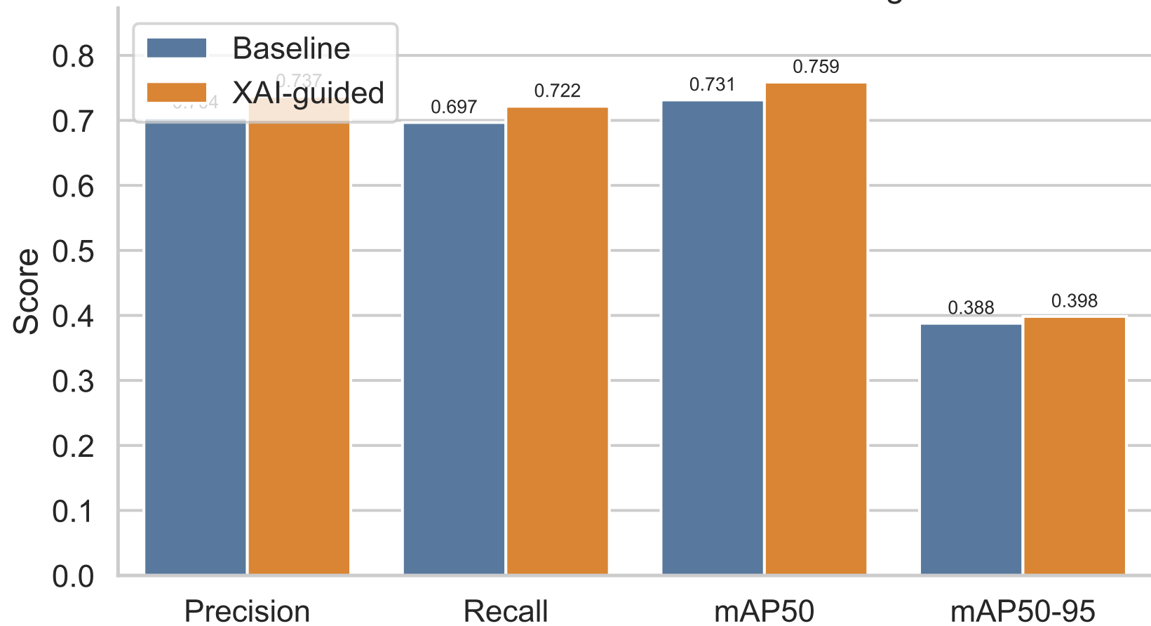
Best validation metrics: Baseline vs XAI-guided
