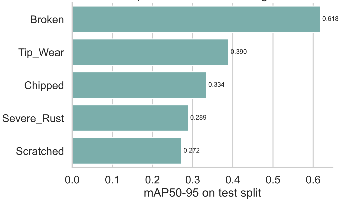
Per-class test performance of the XAI-guided detector
