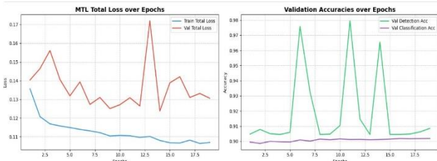
Fig. 4. Training curves for Model 3.
