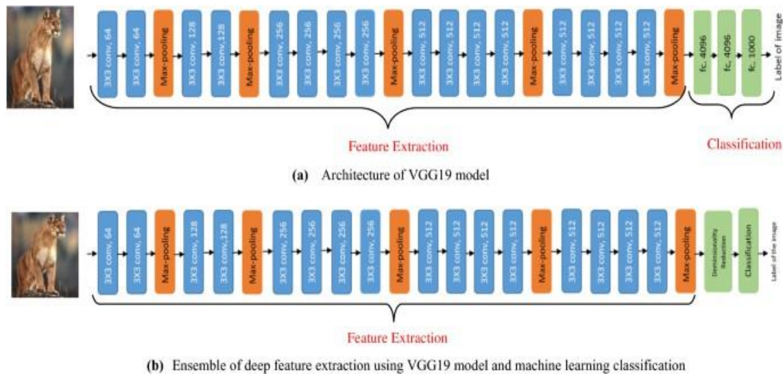
Fig 15. Architecture of VGG-19
