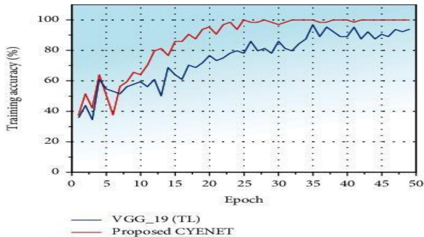
Fig 2. Accuracy for VGG-19 and CYENET.
