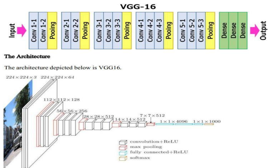
Fig 14. VGG-16 Architecture.
