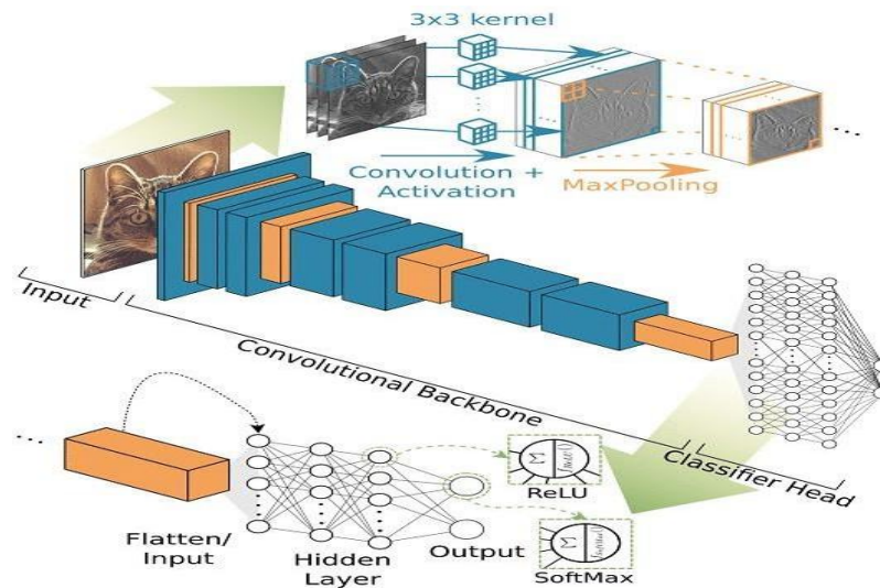
Fig 13. CNN Architecture
