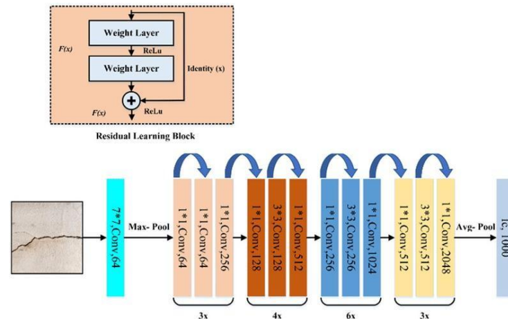
Fig 16. ResNet- 50 Architecture
