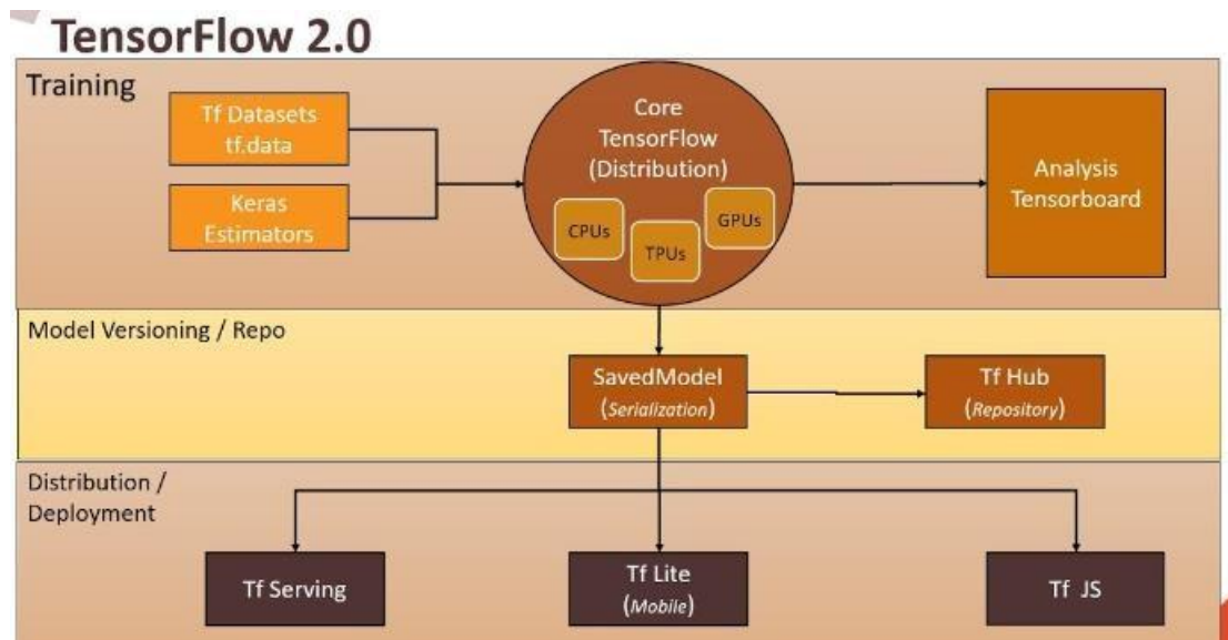
Fig 12. TensorFlow architecture
