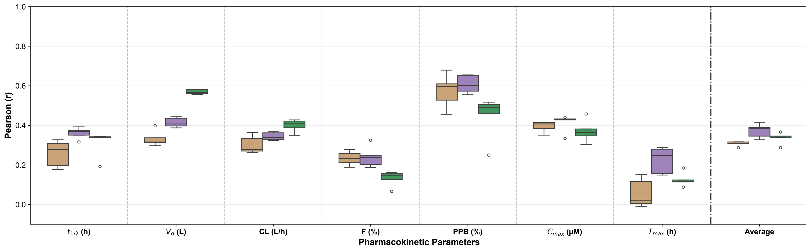
Ensemble Performance on Independent Test Set (Pearson)
