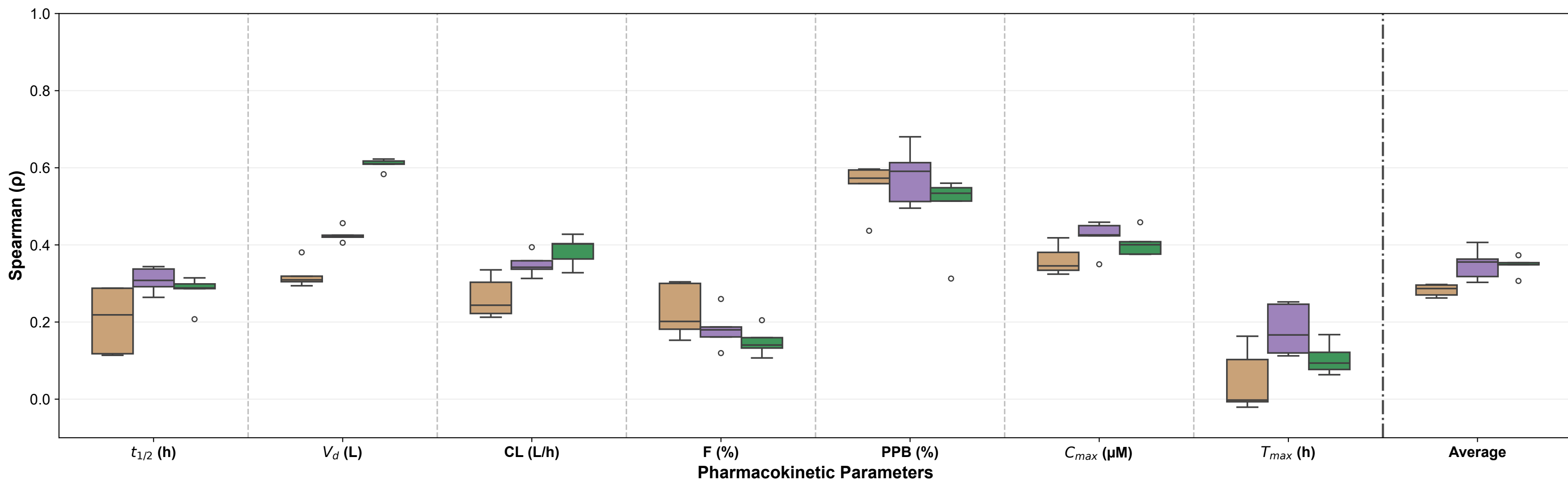
Ensemble Performance on Independent Test Set (Spearman)
