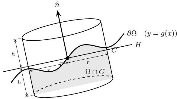
Figure B.1: Cylinder around a boundary point p \in \partial\Omega from definition B.9.1
