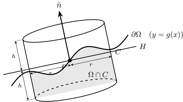
Figure B.1: Cylinder around a boundary point p \in \partial\Omega . See definition B.7.1
