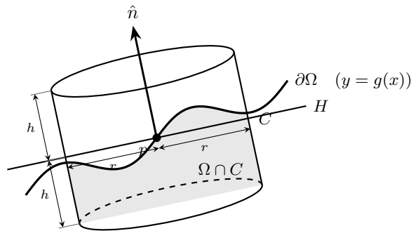
Figure B.1: Cylinder around a boundary point p \in \partial\Omega from definition B.10.1
