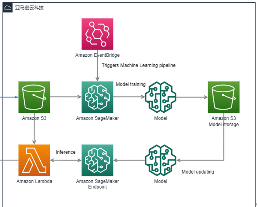
Figure 2. Architecture Diagram of Kingsoft Office's Overseas User Purchase Prediction on Amazon Web Services
