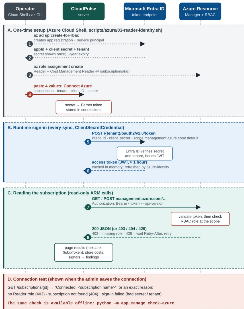
Figure 4.2: Azure credential creation, token acquisition and read-only request sequence
