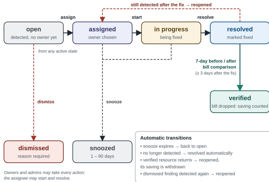
Figure 5.2: Finding lifecycle, with automatic and manual transitions
