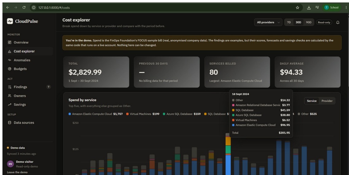
Figure 6.3: Cost explorer with the daily tooltip for 18 September 2024
