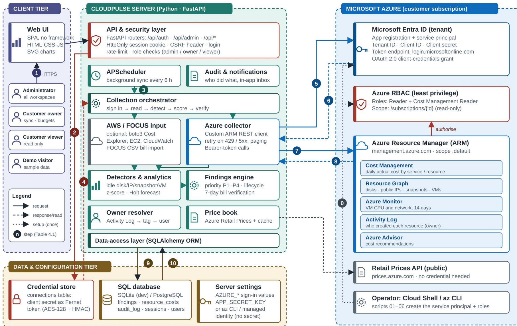
Figure 4.1: CloudPulse system architecture with the Azure credential and data flows
