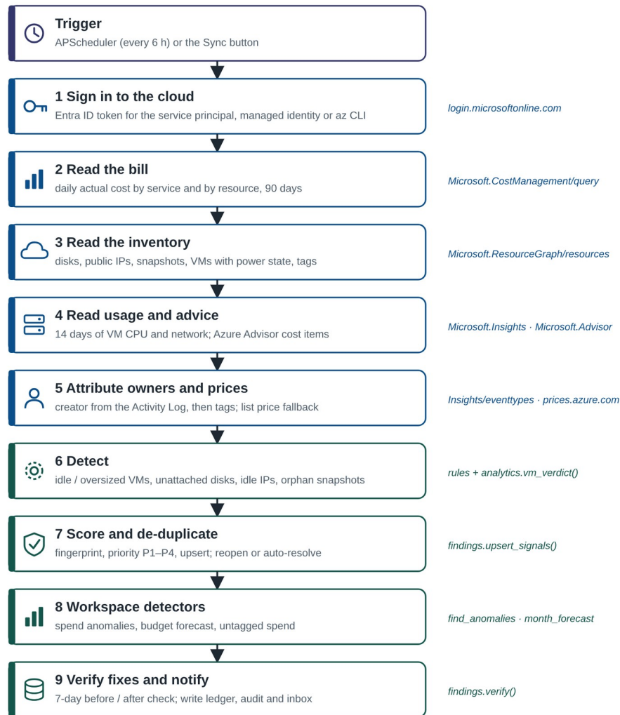
Figure 5.1: The synchronisation pipeline executed on every sync
