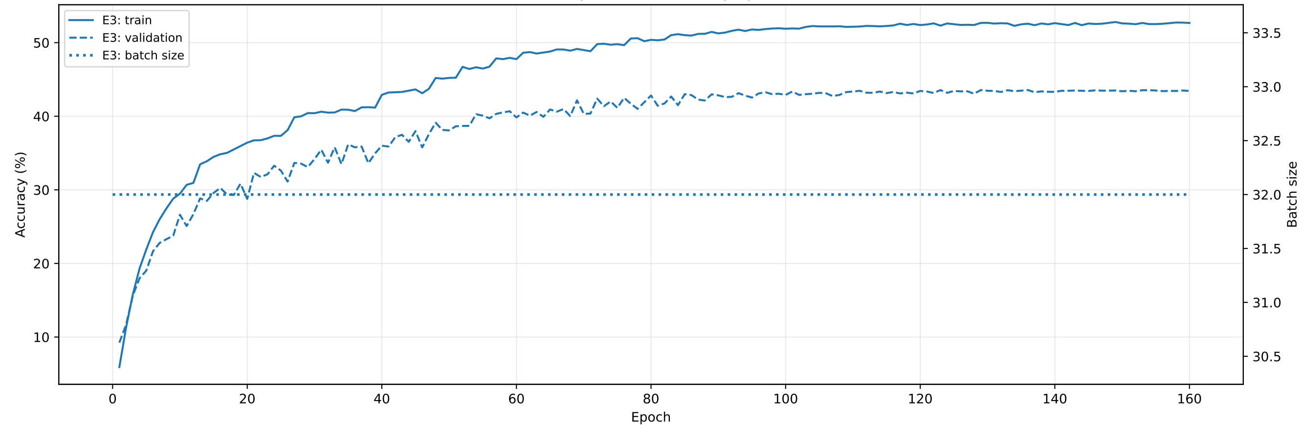
Accuracy and batch size by epoch
