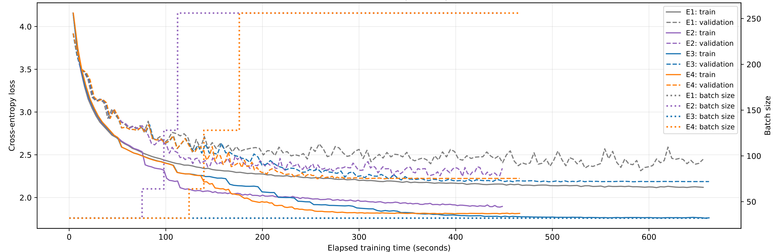
Loss and batch size by training time
